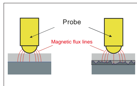
Magnetic flux lines on rough surfaces
