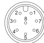
CONN-M12-8F-G
