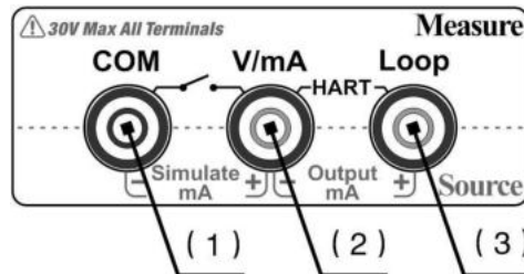
Figure 5 Electric Connection
