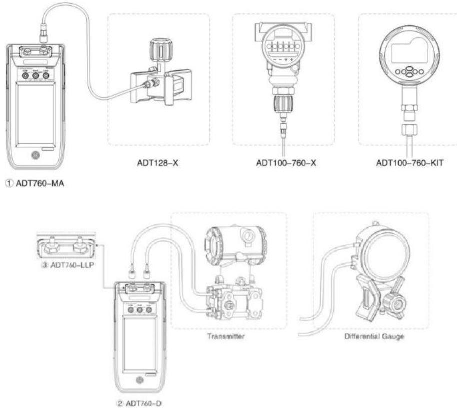
Figure 8 Output Connection
