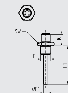
Conector circular, M12 x 1
