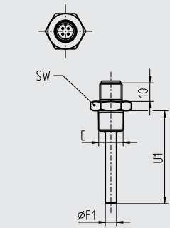
Circular connector M12 x 1
