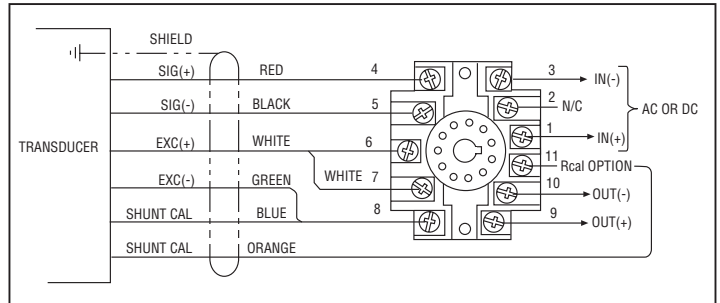
FIGURE 2: Wiring Instructions
